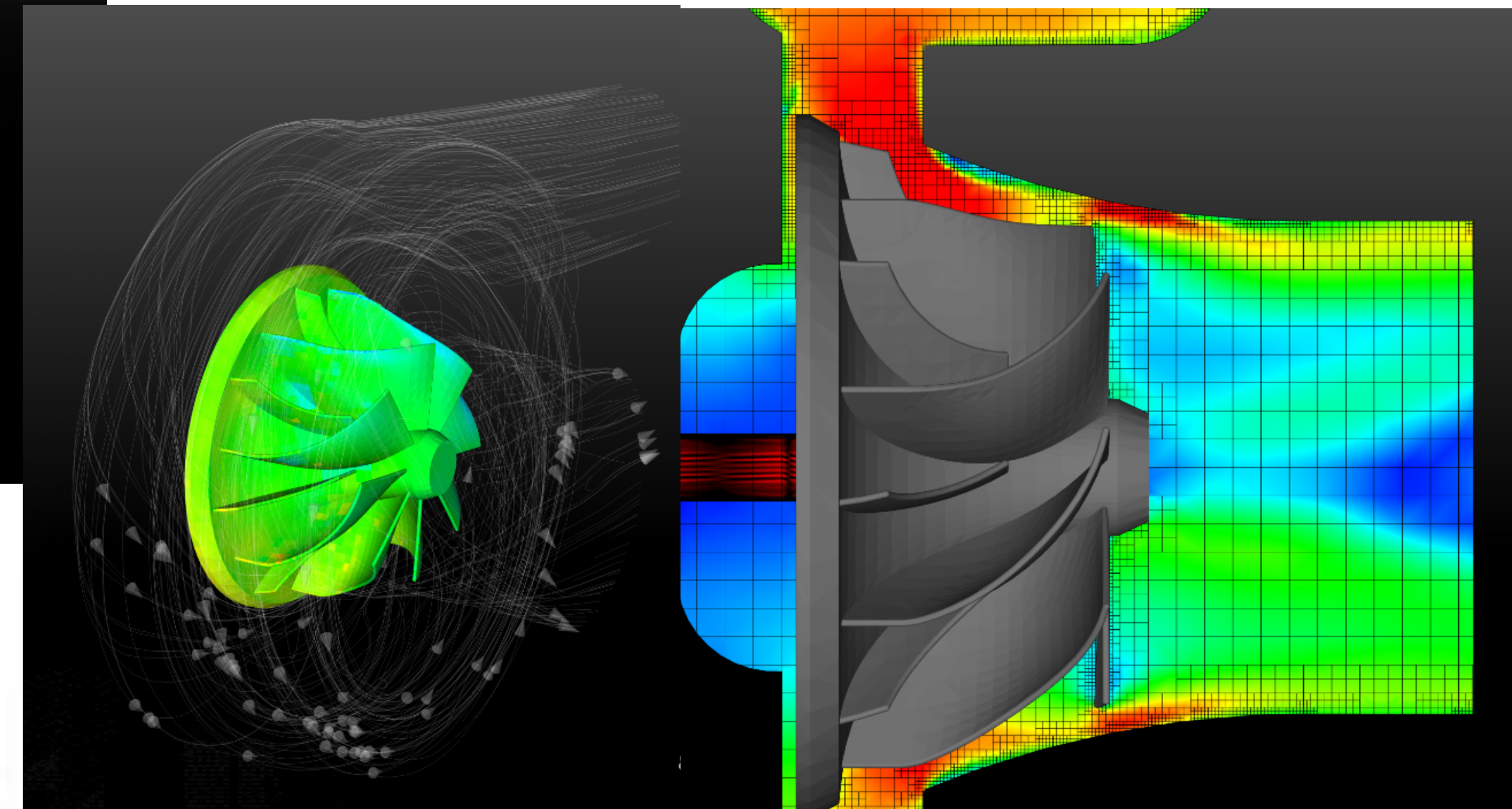
Pressure and Velocity field for turbocharger test case
